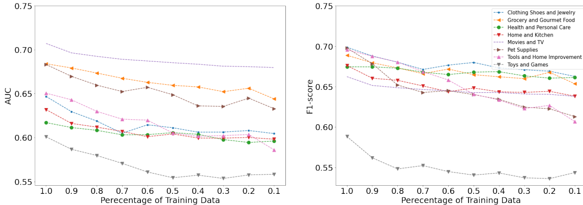
Figure 6.1: Performance of GL-HGCNN trained with different number of training samples. The Y-axis denotes the evaluation metrics and the X-axis denotes the percentage of training samples for training the model.
