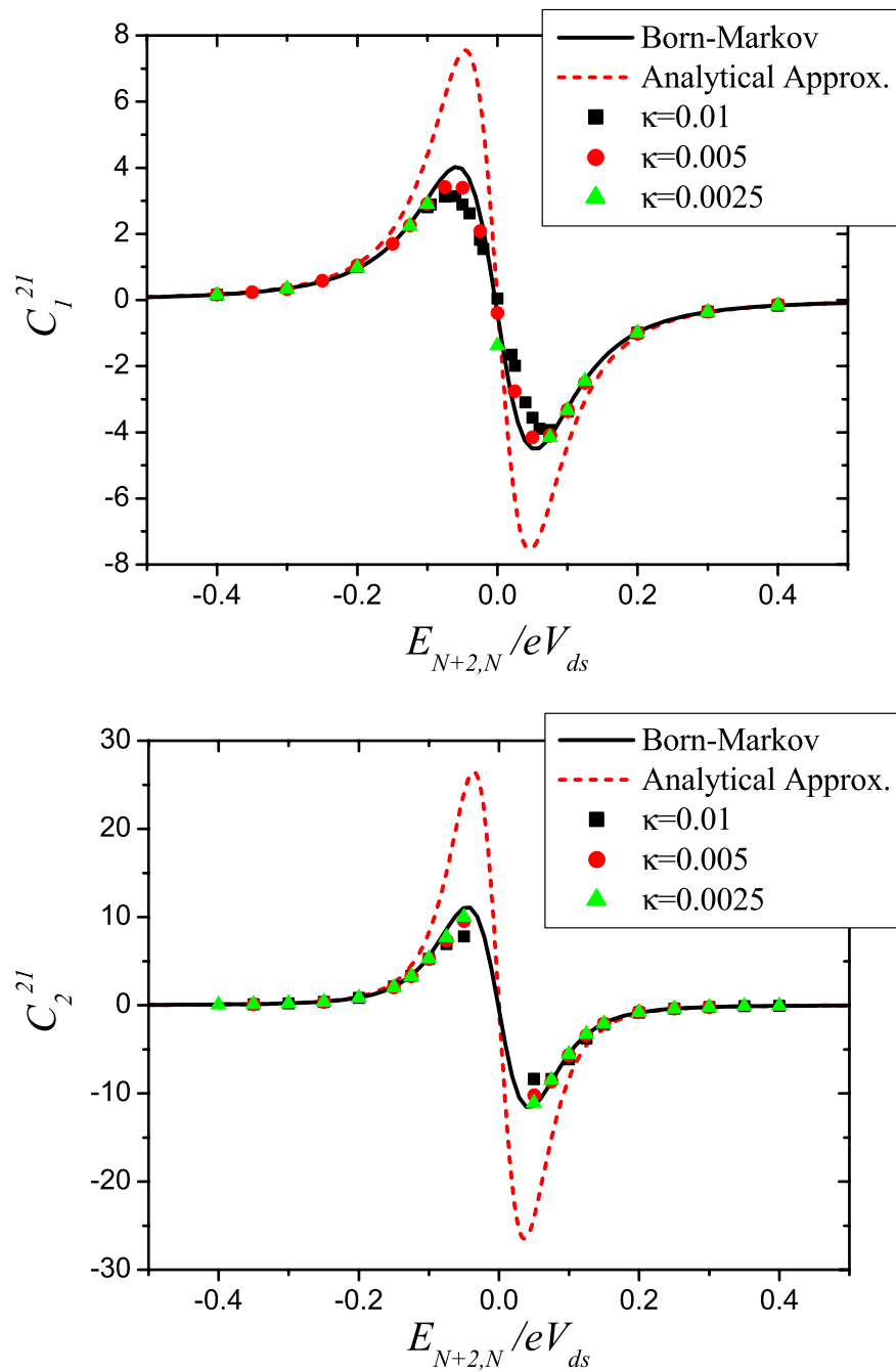
Figure 3. Comparison of numerical calculations of the coefficients C_1^{21} and C_2^{21} with the analytical approximations (equations (21) and (22)). The full curves come from numerical evaluations of equations (15) and (16), whereas the points come from numerical integrations of the master equations (5). For the numerics, we choose \epsilon_J = 1/16 , r = 1 and set the quasi-particle tunnel rates and their gradients to unity. In addition, when integrating the master equations we set \epsilon = 0.1 and vary the value of \kappa as shown.
