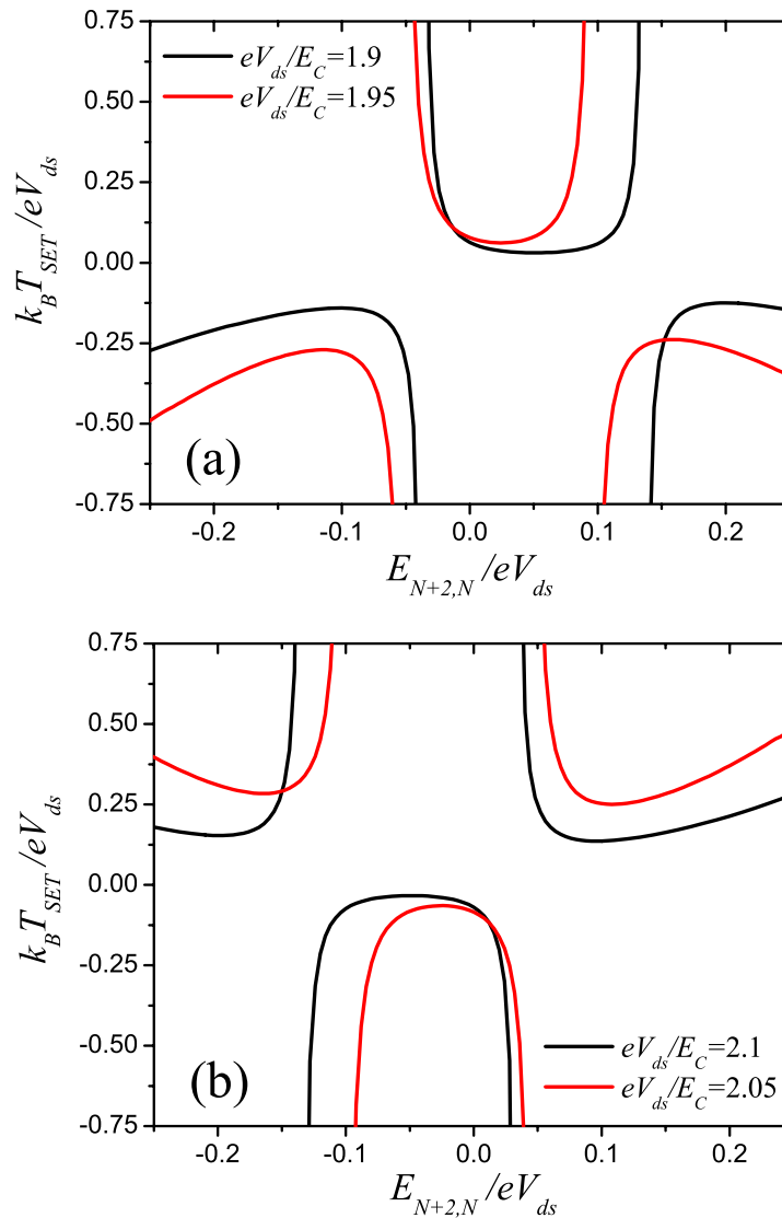
Figure 7. Numerical calculation of T_{SET} (a) below and (b) above the DJQP resonance. The parameters are the same as those used for figure 6.
