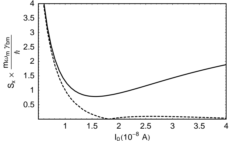
FIG. 2: Displacement detector noise spectral density (solid line) and lower bound (dashed line) versus drive current amplitude. The noise densities are evaluated at \omega = \omega_p + R_\omega \omega_m , corresponding to phase preserving detection.
