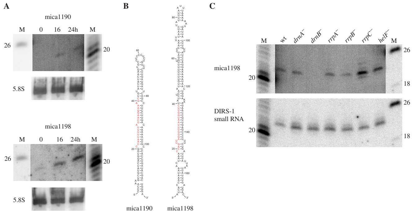
Figure 2. miRNA candidates in D. discoideum (A) northern blot analysis of mica1190 and mica1198 using RNA isolated from growing cells (0 h) and developed cells (16 and 24h). The 5.8S rRNA is used as a loading control and radioactively labeled size markers (M) are shown. (B) Predicted secondary structure (Mfold) of sequences surrounding miRNA candidates mica1190 and mica1198. (C) Northern blot analysis showing the expression of mica1198 in strains where genes encoding putative Dicer homologs ( drnA - and drnB - ), RdRp ( rrpA - , rrpB - and rrpC - ) and RNA helicase ( helF - ) have been disrupted. Wild-type (wt) represents D. discoideum AX2 strain, which is the background strain of all knockout strains except rrpC - . rrpC - was constructed in the AX4 wild-type strain, which displayed similar expression levels as AX2 for all RNAs analyzed in this study (data not shown). The same membrane was stripped and reprobbed with the DIRS-1 small RNA which is expressed approximately equally in all strains analyzed and was therefore used as a loading control.
